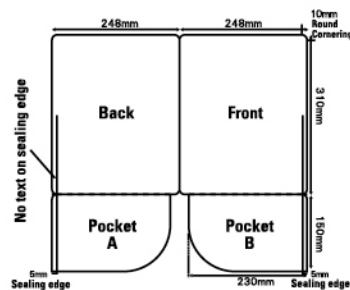
Model PP06 Die-Cutter
