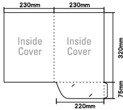
Series B Die-Cutter
