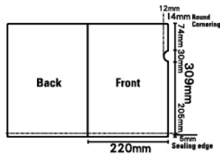
Model PP01 Die-Cutter
