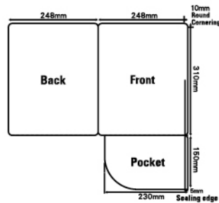
Model PP04 Die-Cutter
