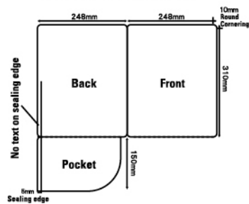
Model PP05 Die-Cutter
