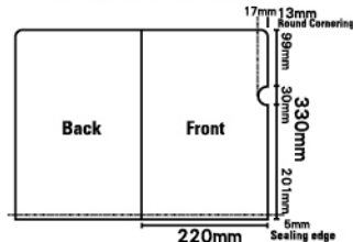
Model PP02 Die-Cutter
