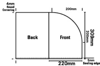
Model PP03 Die-Cutter
