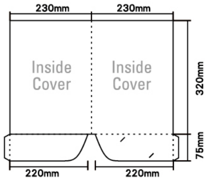
Series A Die-Cutter
