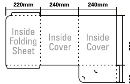
Series G Die-Cutter
