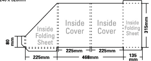
Series H Die-Cutter
