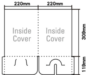
Series C Die-Cutter
